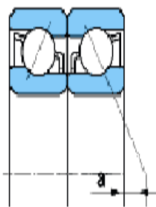
BTB (BACK-TO-BACK)
